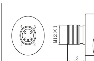
M12航空插件/M12 aviation plug-in
